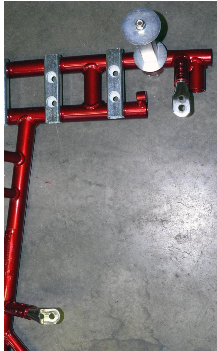
Photo from above of the frame with the section of the two supports for the exhaust system
