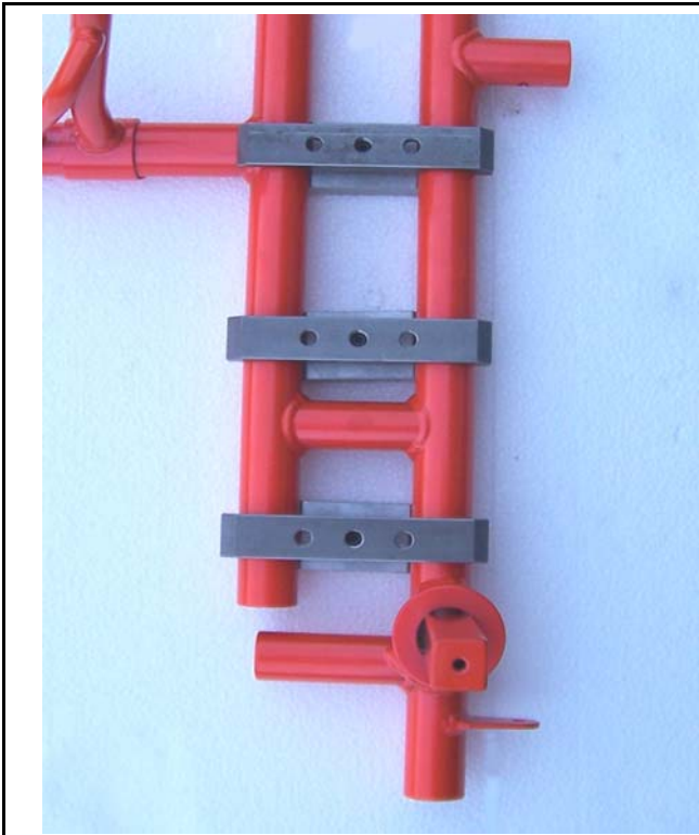
Foto from above of the frame with the section of the engine mount
